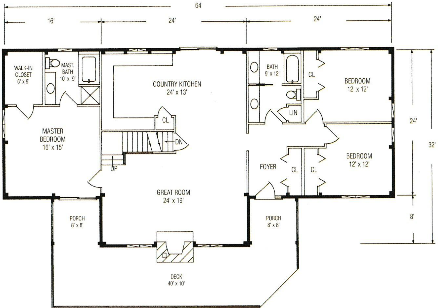
FIRST FLOOR 1,728 SQUARE FEET
