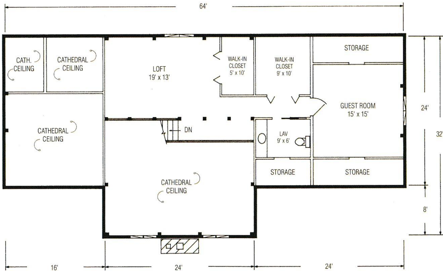
SECOND FLOOR 944 SQUARE FEET
