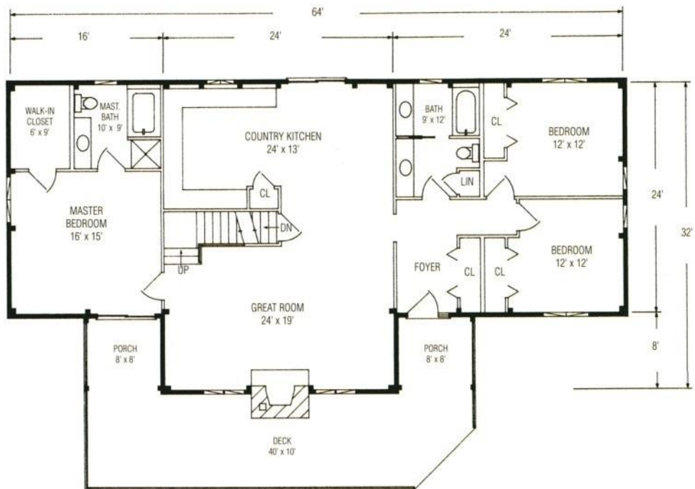
FIRST FLOOR 1,728 SQUARE FEET
