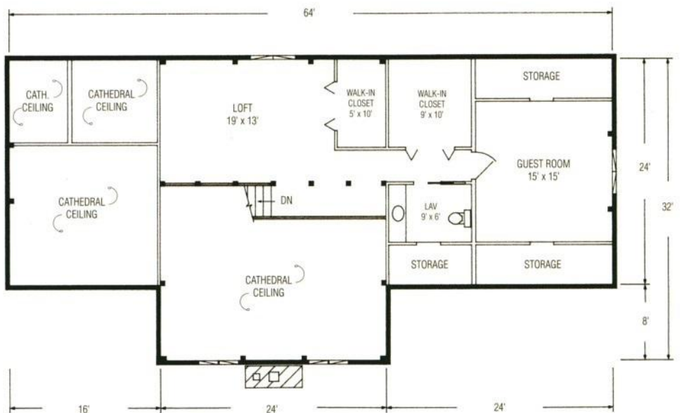
SECOND FLOOR 944 SQUARE FEET
